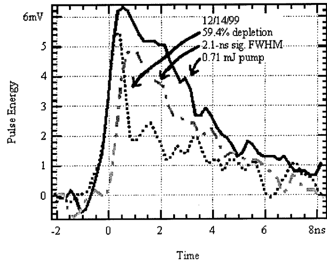
Figure 22. Pump Depletion and Signal Pulse Profile
